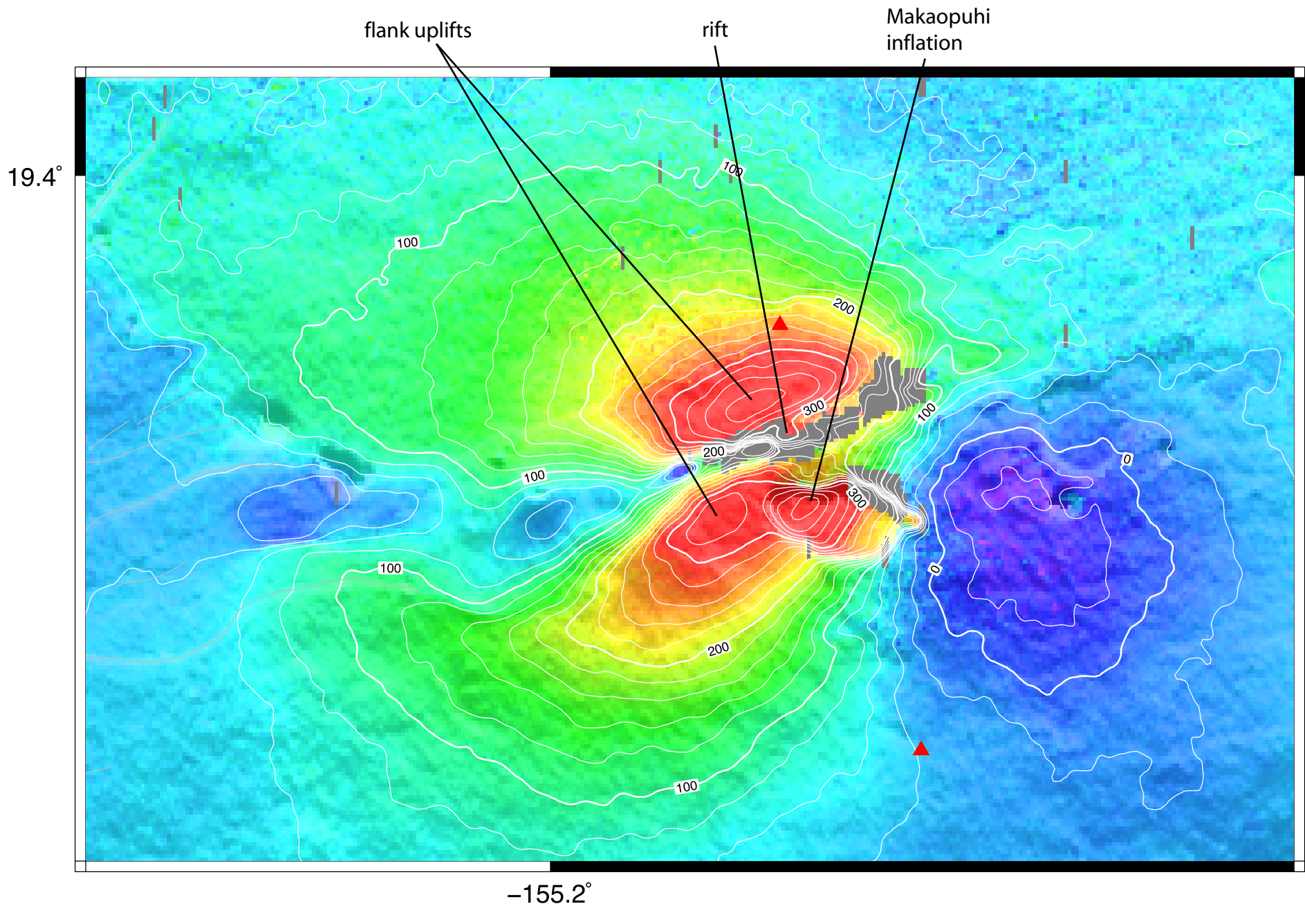
Radar interferogram is zoom from previous figure. Rift-flank uplifts are largely symmetrical while there is a pronounced asymmetry in the rift opening component. The Makaopuhi caldera shows more than 40 mm of local inflation. GPS receivers with continuous vector measurements are marked by red triangles.
